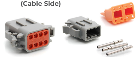
ATM06-08SA Plug (with wedge & contacts shown)
