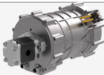
SAE B Mount with Gear Pump
