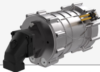
SAE C Mount with Fixed Displacement Piston Pump
