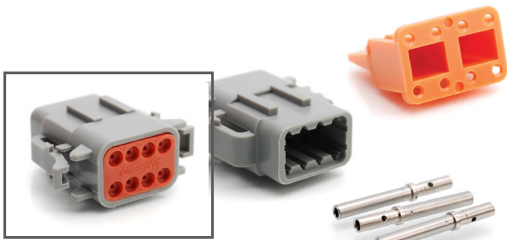
ATM06-08SA Plug (with wedge & contacts shown)
