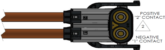
Renhotec Plug Part Number NL1-B060-2AYN-C08
