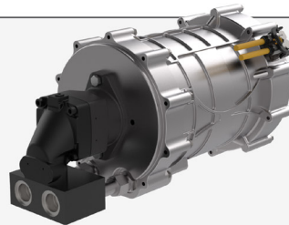
SAE B Mount with Bi-Directional Fixed Displacement Piston
